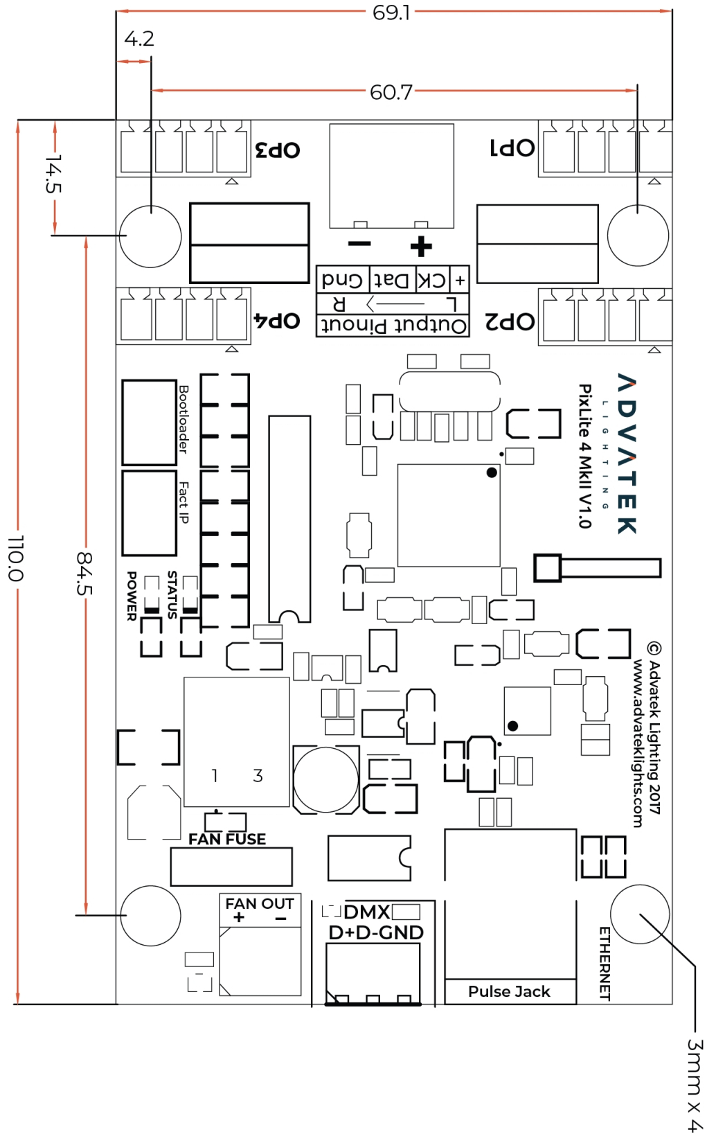
Figure 10: Mechanical Specifications
